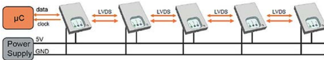
Figure 7: Typical implementation with one master and several slaves
