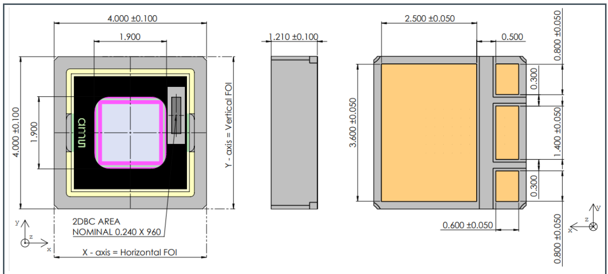
Figure 10: Package Dimensions (1)
